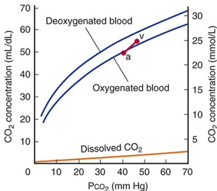
FIGURE 35–5 CO 2 dissociation curves. The arterial point (a) and the venous point (v) indicate the total CO 2 content found in arterial blood and venous blood of normal resting humans. Note the low amount of CO 2 that is dissolved (orange trace) compared to that which can be carried by other means ( Table 35–2 ). (Modified with permission from Schmidt RF, Thews G [editors]: Human Physiology . Springer; 1983.)
