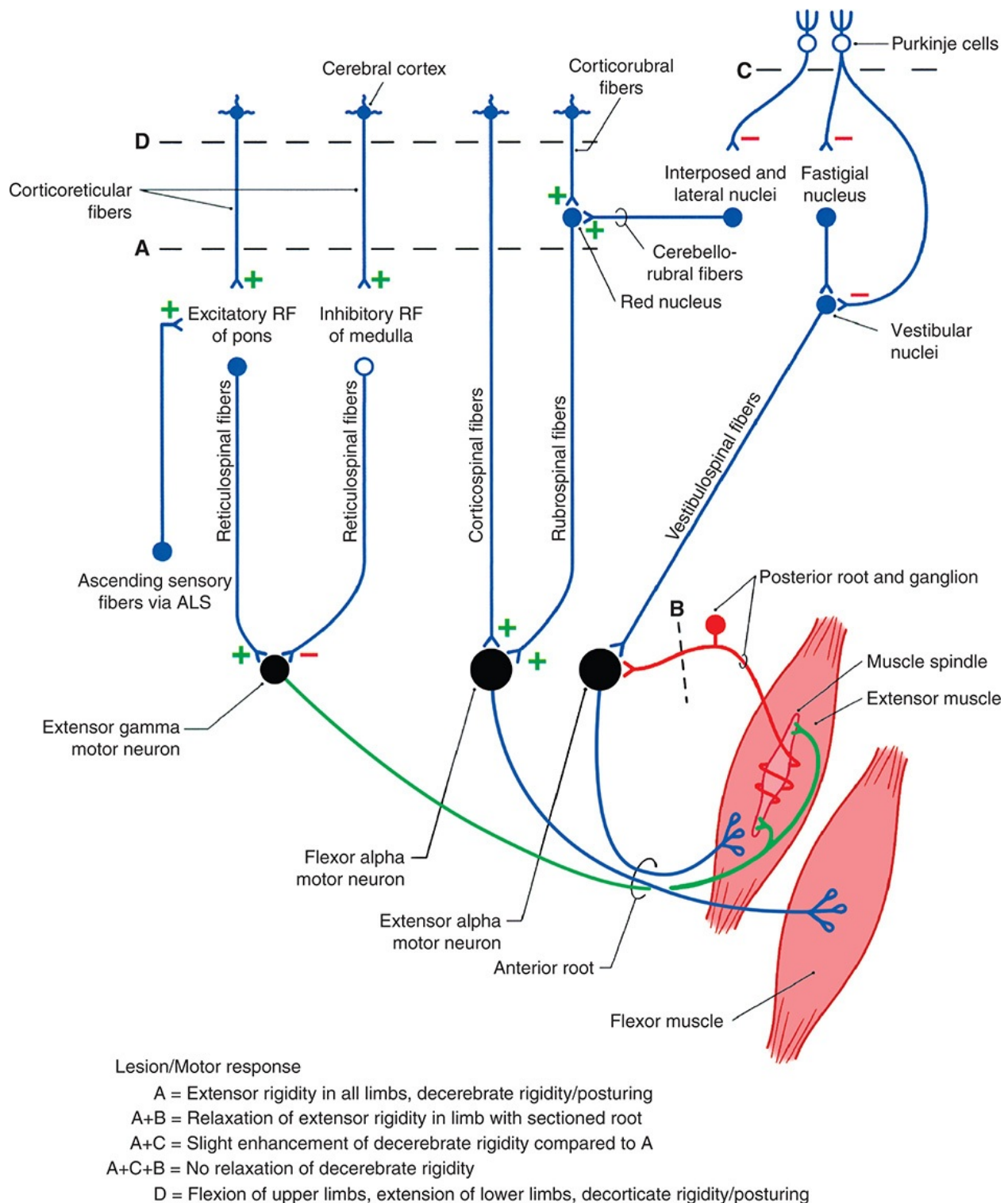
FIGURE 12–11 A circuit drawing representing lesions produced in
