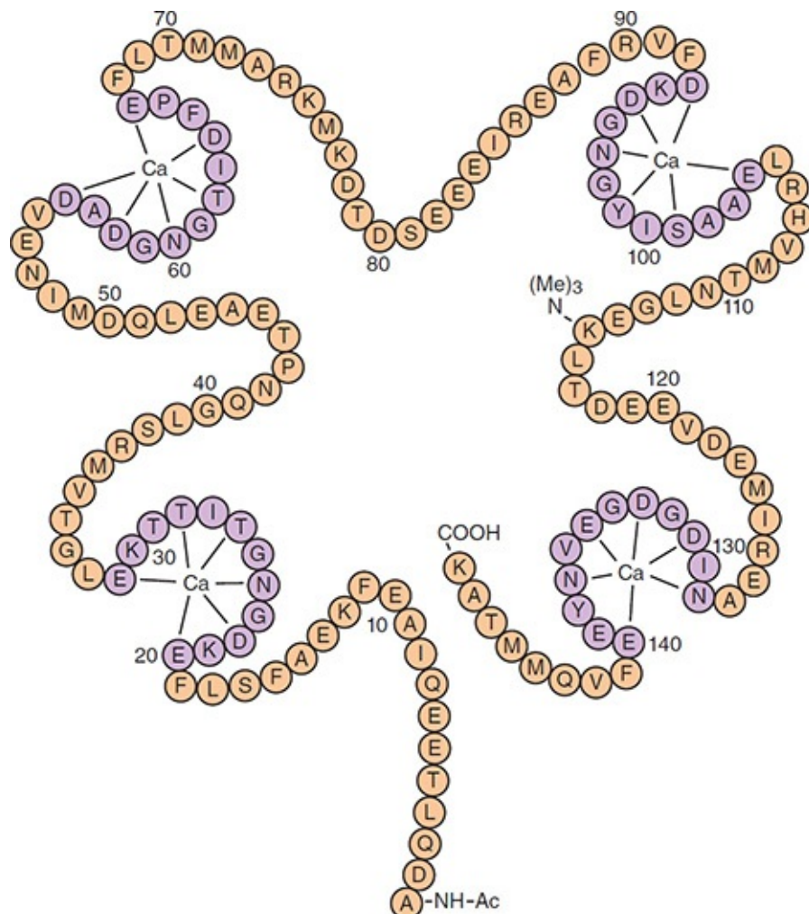
FIGURE 2–23 Secondary structure of calmodulin from bovine brain.
